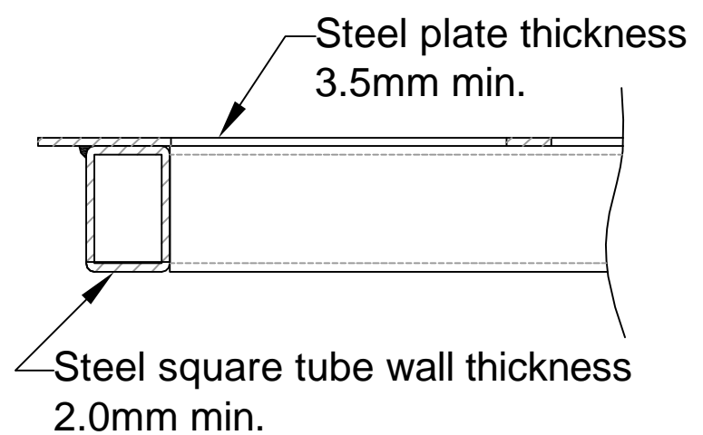
PARTIAL SECTION VIEW
