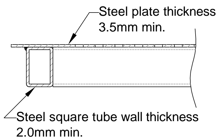
PARTIAL SECTION VIEW
